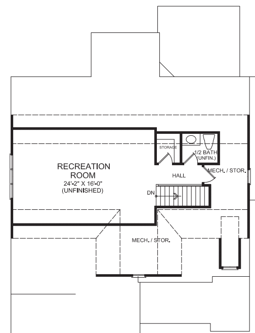
THIRD FLOOR
